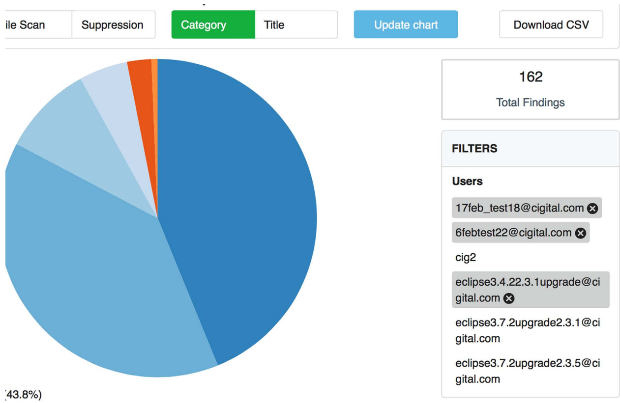
Figure 6, filtering a chart by selecting users. Remember to click the blue “Update” button after selecting new filter criteria.
